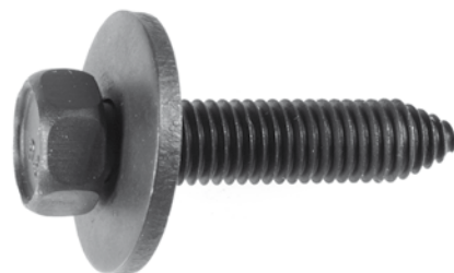
160-176 Phosphate M10-1.50 x 45mm Hex Head Sems * Class 9.8 15mm Hex 30mm (1-3/16") Washer O.D.
